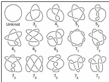
A table of knots. The 'Unknot' was thought to represent hydrogen; to its right, the knot thought to represent carbon. By Jkasd (Own work, Public domain), via Wikimedia Commons "Beautiful Losers: Kelvin's Vortex Atoms", Frank Wilczek (2011) https://www.pbs.org/wgbh/nova/article/beautiful-losers-kelvins-vortex-atoms/
